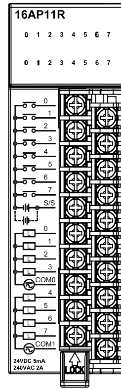
AH16AP11R-5A
