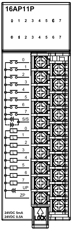
AH16AP11P-5A
