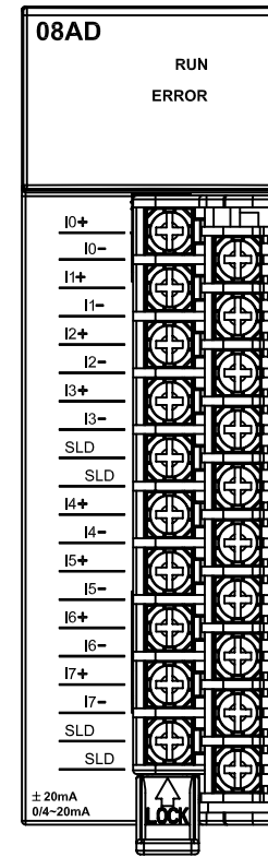
AH08AD-5C
