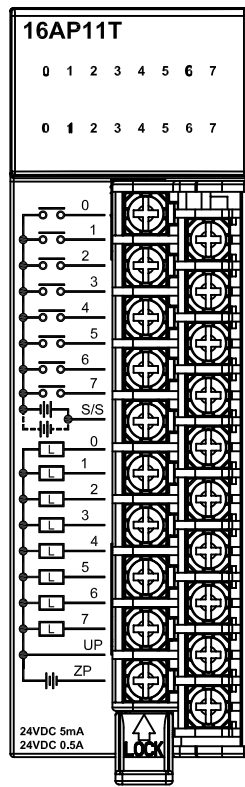
AH16AP11T-5A
