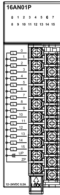
AH16AN01P-5A
