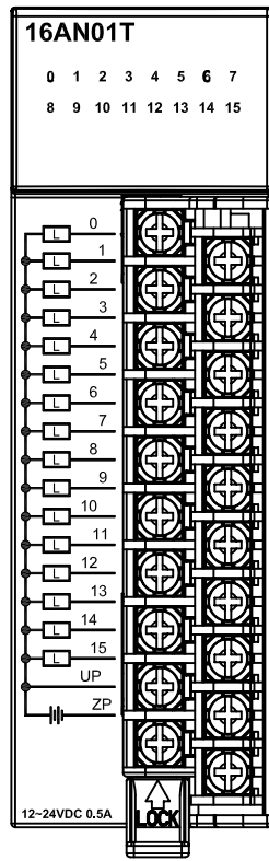
AH16AN01T-5A
