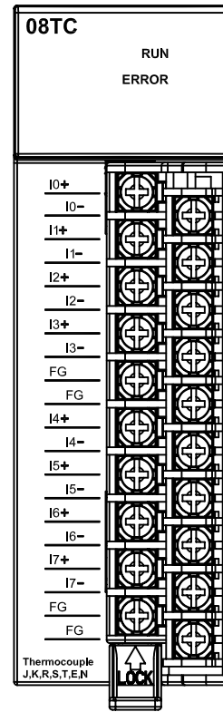
AH08TC-5A
